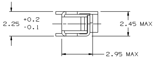
VIEW TO X-X
